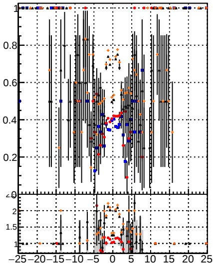
Fake rate vs d BSM Displaced SUSY CKFit BSM Displaced SUSY CKFit BDT
