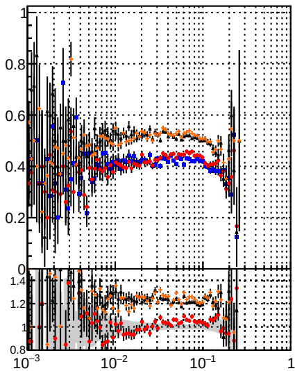
Fake rate vs \epsilon DOM IT CKE BDT DOM IT CKE BDT DOM IT CKE BDT
