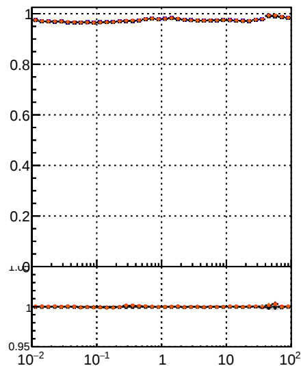
Fake rate vs v — DOM TT CKE — DOM TT CKE fit — DOM TT BDT — DOM TT mkFit
