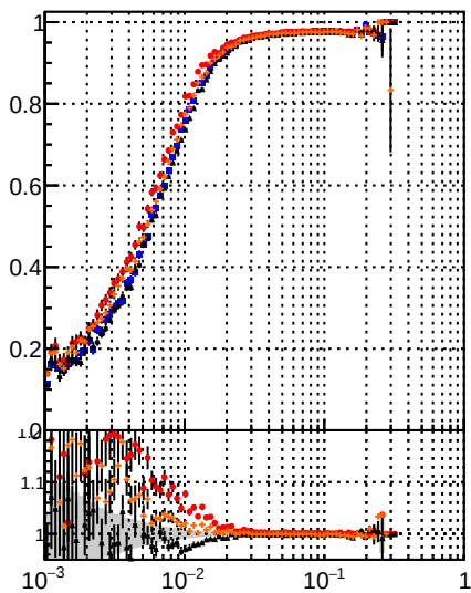
Fake rate vs \frac{dr}{dr_{max}} Legend: DOM IT CKE CKE fit BDT BDT fit
