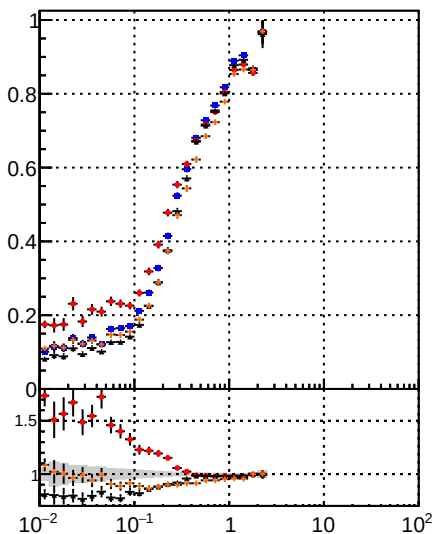
Legend for Fake rate vs. sim PV z: DOM (blue circles) CKE (red crosses) BDT (black dots) DOM (orange circles) CKE (red crosses) BDT (black dots) DOM (green circles) CKE (red crosses) BDT (black dots)
