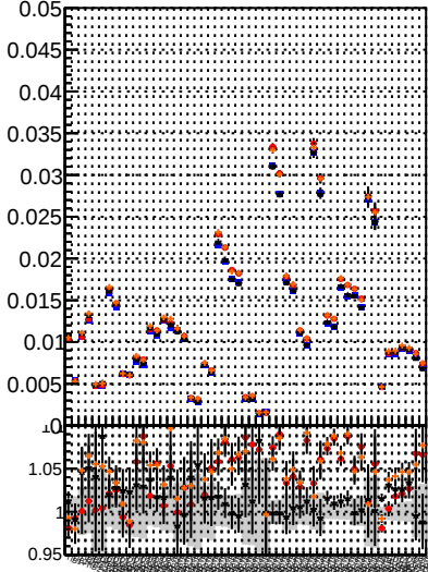
Fake rate vs. BGM IT SKE CRFit BDT CRFit BDT
