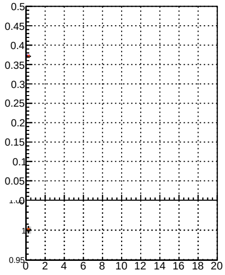
Fake rate vs. \chi^2 for BSM, CKFit, BDT, and BSM+CKFit+BDT
