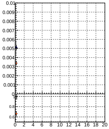
Fake rate vs. \chi^2 for BSM, CKFit, BDT, and BSM+CKFit+BDT
