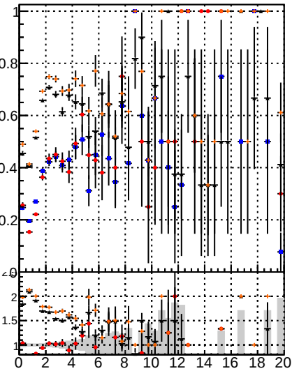
Fake rate vs. BGM CKE BDT CKEfit BDT BDT BDT BDT BDT
