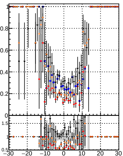
Fake rate vs d BSM CKFit CKFit+BDT CKFit+BDT+INR BSM CKFit CKFit+BDT CKFit+BDT+INR
