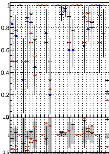
Fake rate vs. BSM CKFit CKFit_BDT BSM CKFit CKFit_BDT
