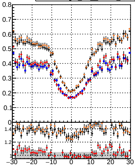
DOM TT CKE TT TT TT DOM TT mkeFit BDT Fake rate vs vertpos
