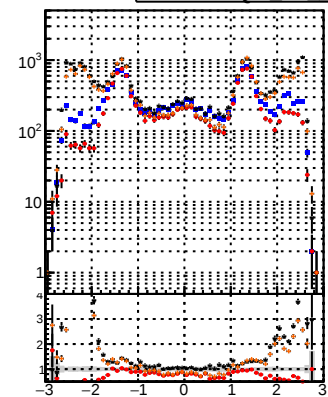
N of reco track vs \eta Legend: BQM, TT, CKFit, BDT
