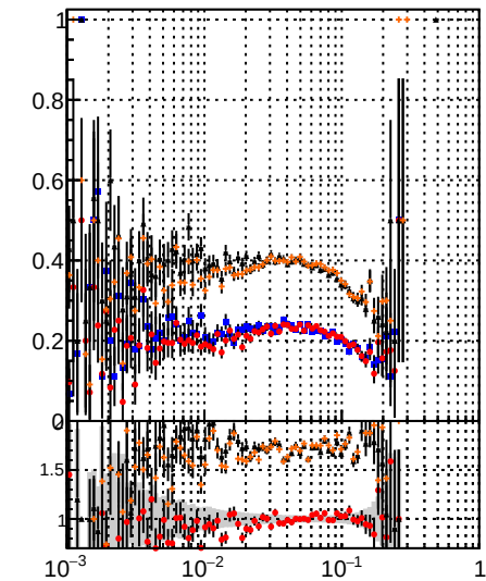
Fake rate vs \epsilon Method Line Style Marker Fit DOM Solid Blue square CKE IT Dashed Red circle mkFit BDT Dotted Black triangle BDT
