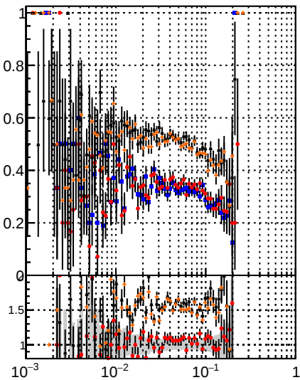
Fake rate vs \epsilon Series Symbol Line Style Color DOM circle Solid Black IT circle Solid Blue CKE circle Solid Red CKE fit circle Solid Orange BDT circle Solid Grey BDT fit circle Solid Light Grey BDT fit circle Dashed Light Grey BDT fit circle Dotted Light Grey
