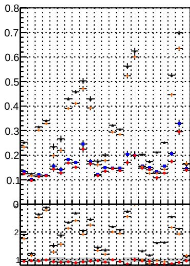
Fake rate vs. BGM SKE CRF BDT mkrFit BGM SKE CRF BDT mkrFit
