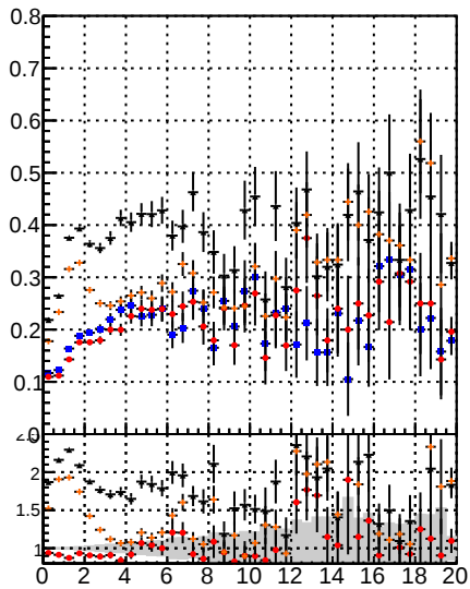
Fake rate vs. BGM SKE CRF BDT mkrFit BGM SKE CRF BDT mkrFit
