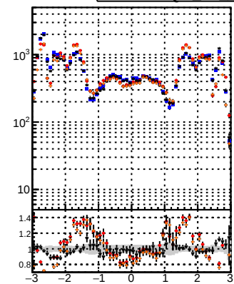
N of reco track vs \eta Legend: BQM TT CKE BDT BQM TT CKE BDT
