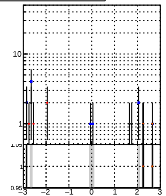
N of associated (recoToSim) duplicate tracks vs \eta Legend: BQM TT CKE BDT
