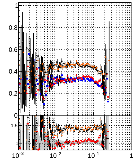
Fake rate vs \epsilon DOM IT CKE CKEfit BDT mkFit
