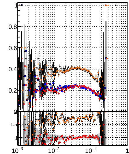
Fake rate vs \epsilon Method Line Style Marker Color DOM Solid None Black IT Solid None Blue CKE Solid None Red mkFit Solid None Orange BDT Dashed None Black CKE fit Dashed None Red BDT fit Dashed None Blue
