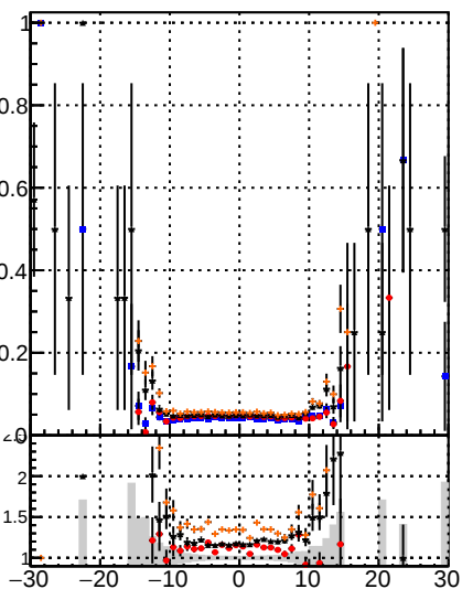
Fake rate vs d BSM SKE CKE BDT BSM SKE CKE BDT
