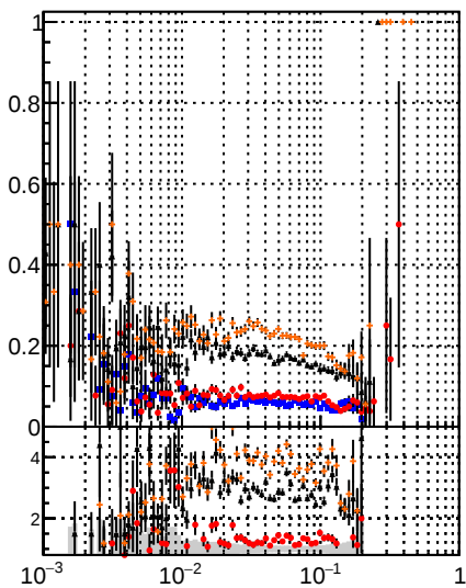
Fake rate vs \epsilon Legend: DOM IT CKE DOM IT CKE fit DOM IT mkFit BDT
