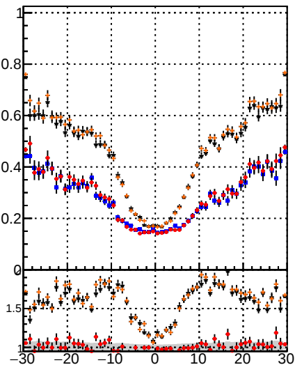
Legend for Fake rate vs vertpos: DOM IT CKE BDT DOM IT CKE BDT DOM IT CKE BDT
