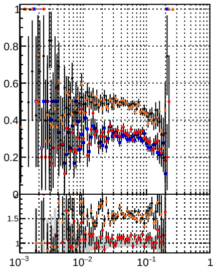
Fake rate vs \epsilon DOM IT CKE CKE fit BDT DOM IT CKE CKE fit BDT DOM IT CKE CKE fit BDT
