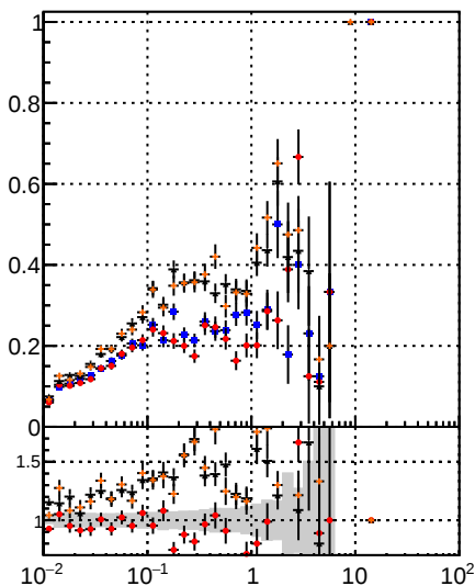
Fake rate vs v —■— DOM IT CKE —●— DOM IT CKE fit —★— DOM IT CKE fit BDT —×— DOM IT mktFit BDT
