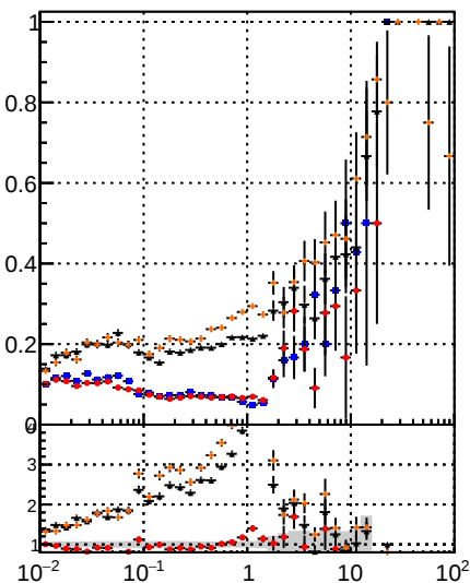
Fake rate vs v Legend: DOM TT CKE CKE fit BDT mke fit
