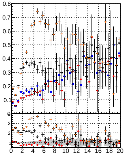
Fake rate vs. BQM IT SKE BDT BQM IT SKE BDT
