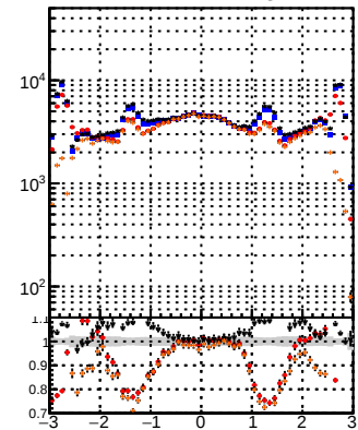
N of reco track vs \eta Legend: BQM (blue circles), TT (black crosses), CKEfit (red stars), BDT (orange dots)
