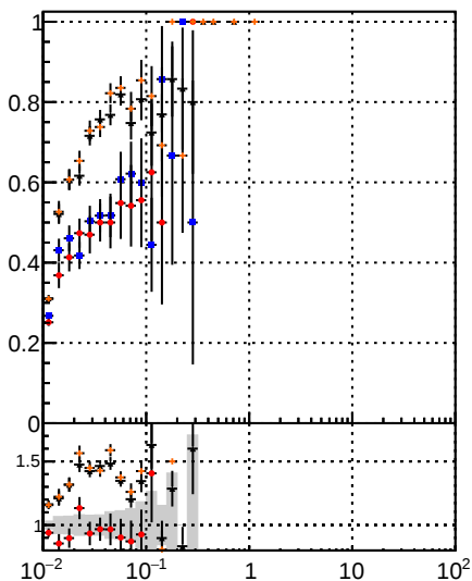
Legend for Fake rate vs v: DOM (blue squares) CKE (orange crosses) BDT (red stars) mktFit (black dots)
