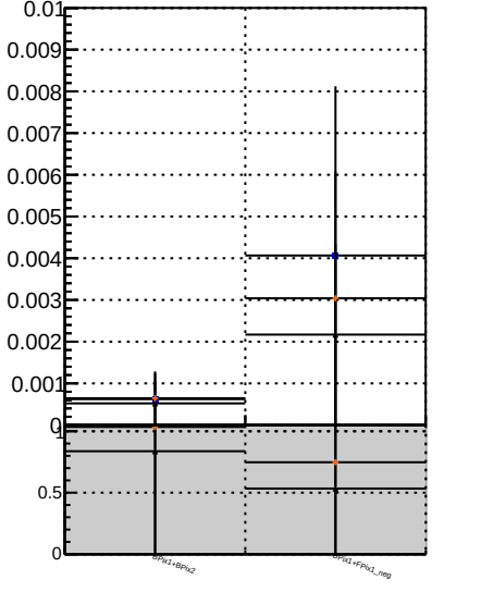
Fake rate vs. BDT CKFit SKFit BDT CKFit SKFit
