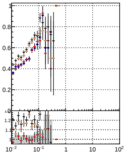
Fake rate vs v_z Legend: DOM (black) IT (blue) CKE (red) CKEfit (orange) BDT (grey) mkefit (green)
