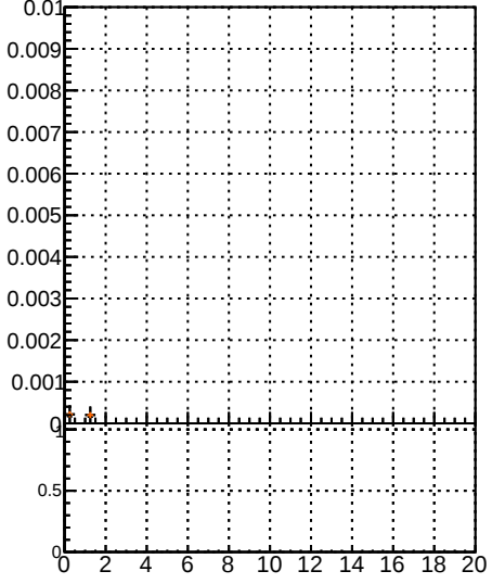
Fake rate vs. BDT SKE CKFit BDT BDT SKE CKFit BDT BDT SKE CKFit BDT
