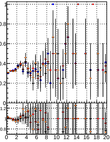
Fake rate vs. BDT SKE CKFit BDT BDT SKE CKFit BDT BDT SKE CKFit BDT
