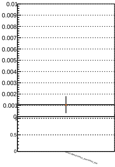
Fake rate vs. BDT SKE CKFit BDT BDT SKE CKFit BDT BDT SKE CKFit BDT
