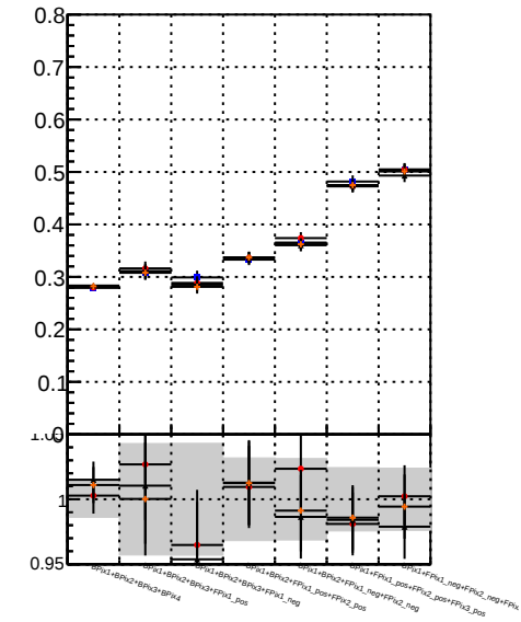
Fake rate vs. BDT SKE CKFit BDT BDT SKE CKFit BDT BDT SKE CKFit BDT
