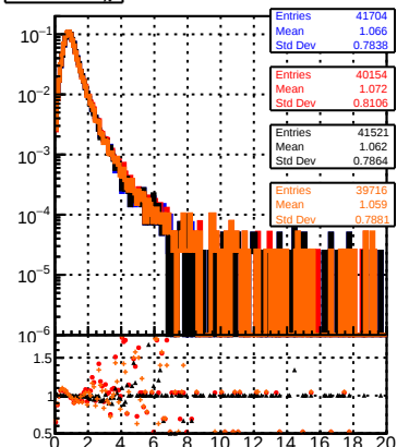
Legend: DQM_TT_CKF_ DQM_TT_mkFit_ DQM_TT_CKF_BDT_ DQM_TT_mkFit_BDT_
