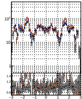
N of reco track vs \eta Legend: BQM (blue circles), TT (black squares), CKEfit (red stars), BDT (orange triangles)
