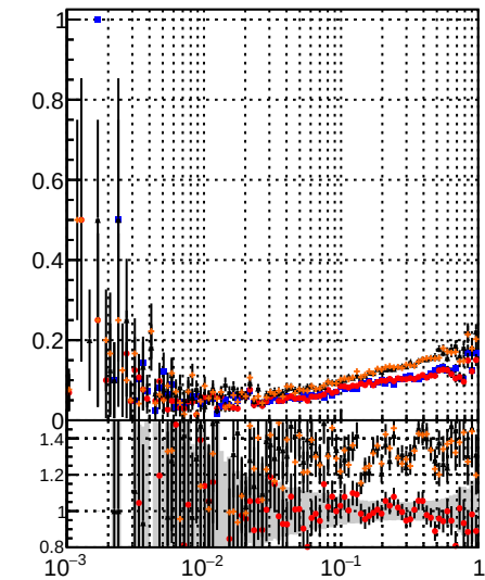
Fake rate vs \frac{dr}{pu} Legend: DOM TT CKE CKE fit BDT DOM TT CKE CKE fit BDT DOM TT CKE CKE fit BDT
