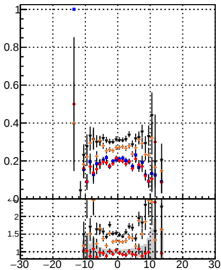
Fake rate vs v Legend: DOM IT CKE CKEfit BDT mkFit
