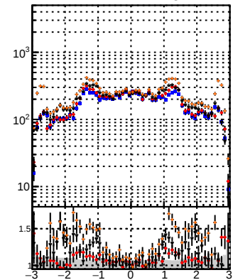
N of reco track vs \eta Legend: \square BSM, \square CKFit, \square mrFit, \square BDT
