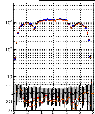
N of reco track vs \eta Legend: BQM, TT, CKEFit, BDT, mkrFit, BDT
