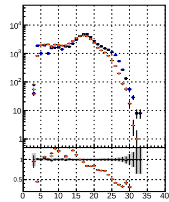
DOM TT CKE DOM TT mkt BDT N of reco track vs hit
