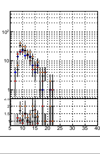
N of associated (recoToSim) duplicate tracks vs hit
