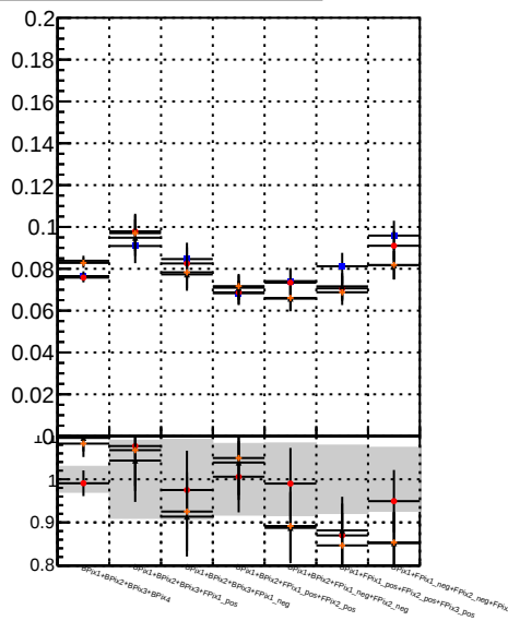
Fake rate vs. BGM CKF BDT mkrFit BDT
