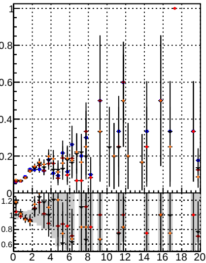
Fake rate vs. BGM CKF BDT mkrFit BDT
