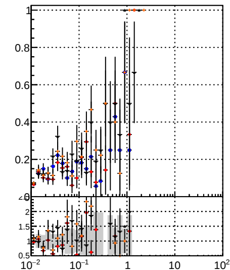
Fake rate vs v DOM IT CKE IT CKE BDT BDT CKE BDT BDT CKE BDT
