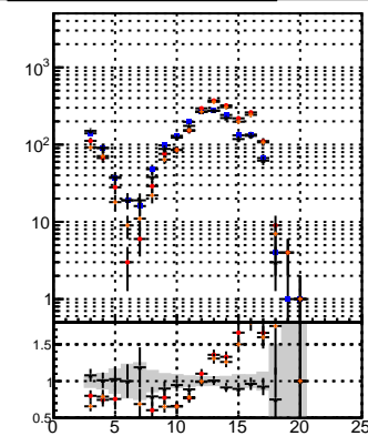
Fit BDT
