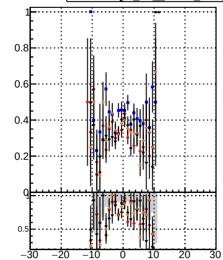
DOM CKE CKE fit BDT Fake rate vs v
