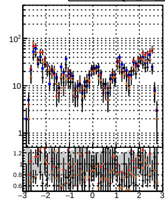
N of reco track vs \eta Legend: BQM, TT, GKF, mkFit, BDT
