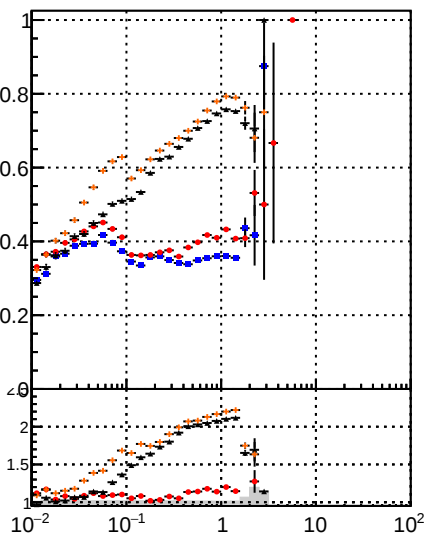
Legend for Fake rate vs v: DOM IT CKE BDT DOM IT CKE BDT DOM IT CKE BDT
