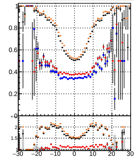
Legend for Fake rate vs v: DOM IT CKE BDT DOM IT CKE BDT DOM IT CKE BDT
