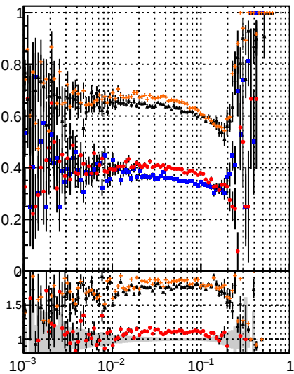
Fake rate vs \mu Legend: DOM, IT, CKE, mkFit, BDT
