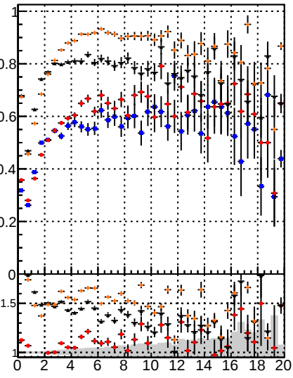
Fake rate vs. BSM CKF CKF+BDT BSM CKF CKF+BDT
