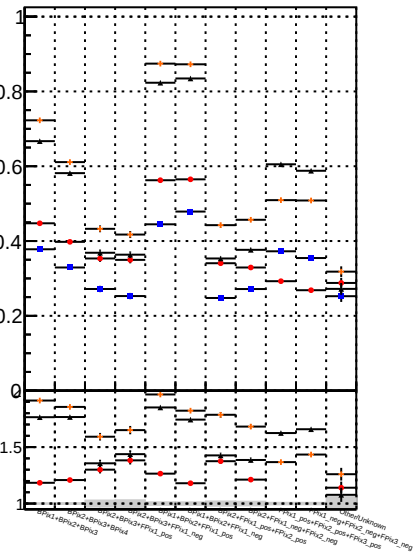
Fake rate vs. BSM CKF CKF+BDT BSM CKF CKF+BDT
