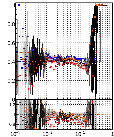
Fake rate vs \epsilon DOM IT CKE BDT DOM IT CKE BDT DOM IT CKE BDT DOM IT CKE BDT
