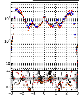
N of reco track vs \eta Legend: BQM, TT, CKEfit, BDT, mkFit
