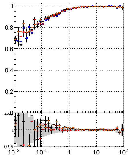
Fake rate vs v —■— DOM IT CKE —●— DOM IT CKE —▲— DOM IT CKE —× BDT
