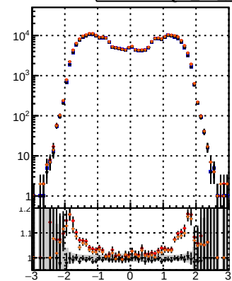
N of reco track vs \eta Legend: BQM, CKFit, mkrFit, BDT
